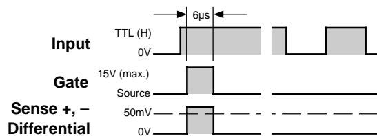
Timing Diagram 3. Fault Condition, C_T = \text{Grounded}
