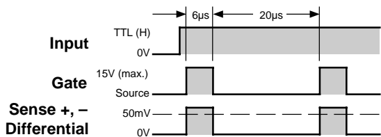
Timing Diagram 2. Fault Condition, C_T = \text{Open}
