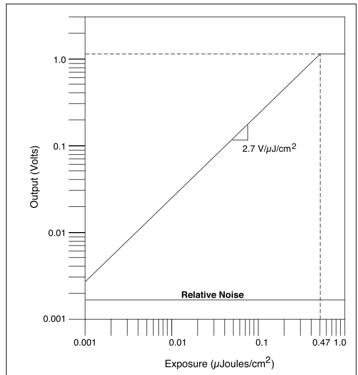
Figure 8. Typical Transfer Characteristics
