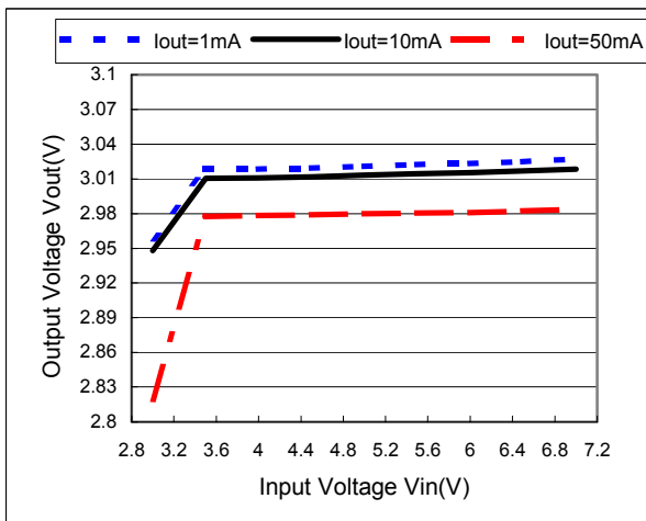
6.4.6. Output voltage vs. input voltage (Vout = 3.0V)
