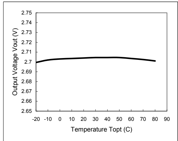
6.4.11. Output voltage vs. temperature (Vout = 2.7V)
