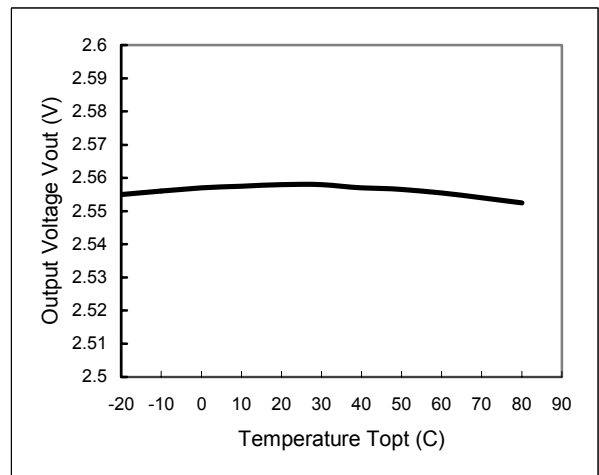
6.4.12. Output voltage vs. Temperature (Vout = 2.55V)
