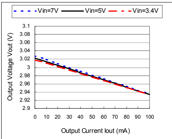
6.4.2. Output voltage vs. output current (Vout = 3.0V)
