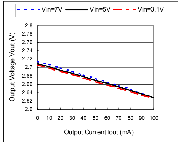
6.4.3. Output voltage vs. output current (Vout = 2.7V)
