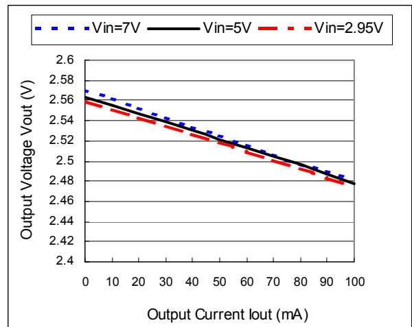
6.4.4. Output voltage vs. output current (Vout = 2.55V)
