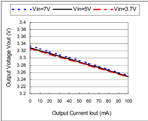
6.4.1. Output voltage vs. output current (Vout = 3.3V)
