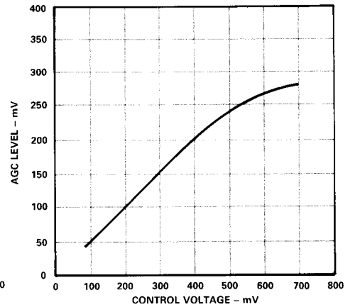
Figure 6. AGC Level vs. Control Voltage
