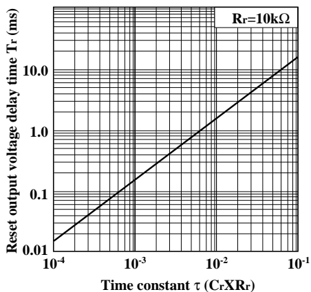
Fig.13 Reset Output Delay Time vs. Time Constant
