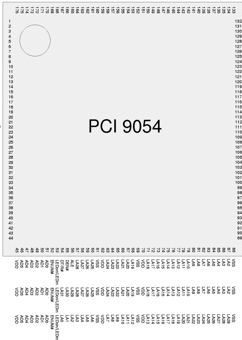
Figure 14-3. 176-Pin PQFP PCI 9054 Pinout
