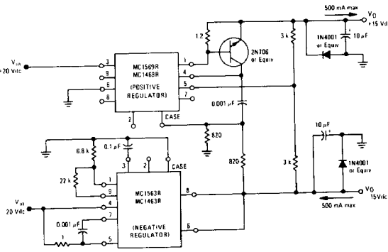
FIGURE 3 - ±15 V, ±400 mA COMPLEMENTARY TRACKING VOLTAGE REGULATOR
