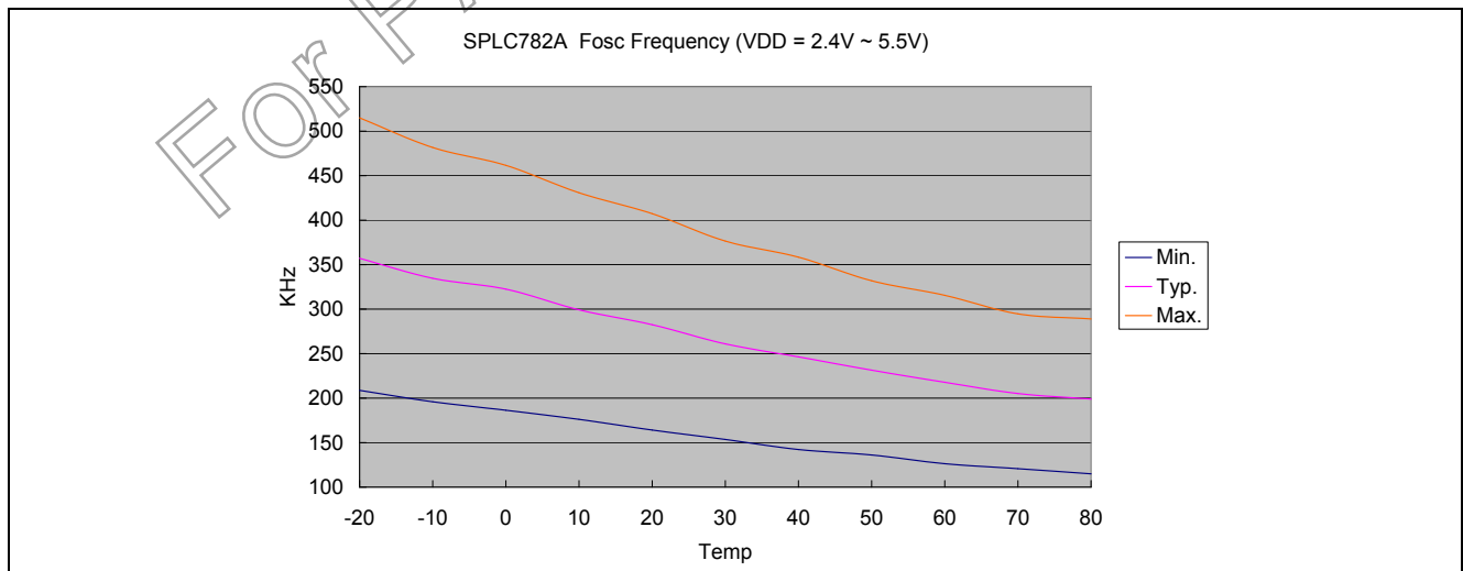
Figure 6-3: The Relationship Between Fosc and Temperature
