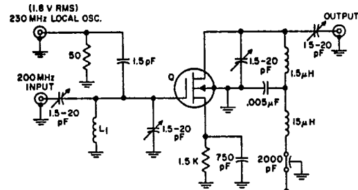
Fig.3 - Conversion Power Gain Test Circuit.
