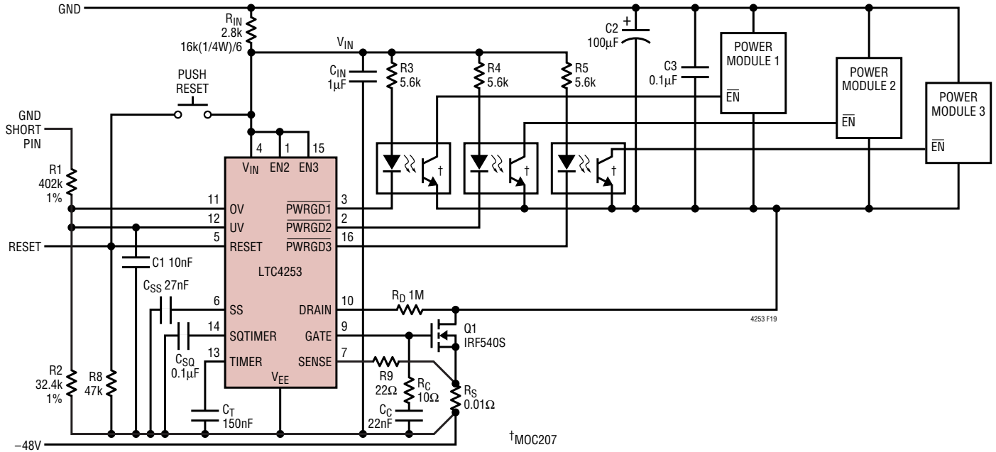
Figure 19. -48V/5A Application Sequenced Without Optical Feedback
