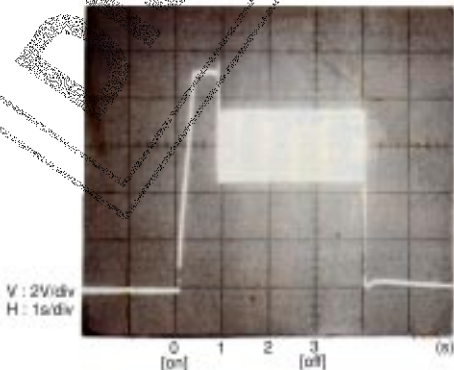
(1) C_{NF}=100\mu F , perfect discharge
