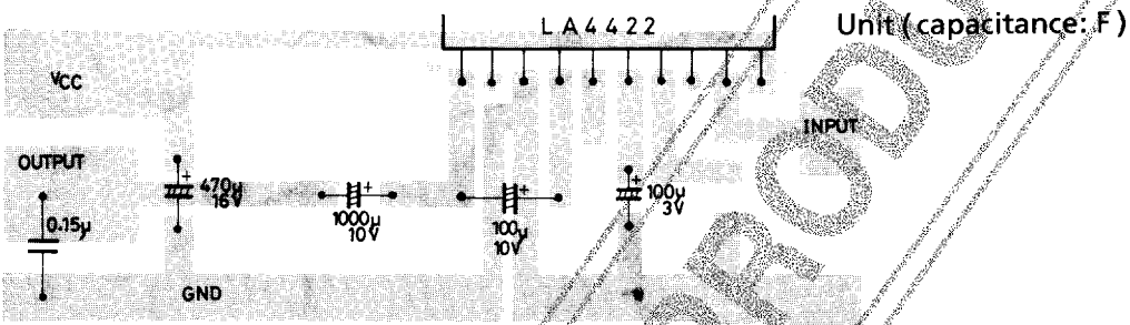
Printed Circuit Pattern (22x65mm 2 , Cu-foiled side)
