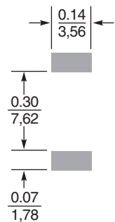
Recommended Land Pattern
