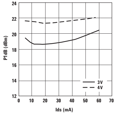
Figure 13. P1dB vs. Idsq and Vds Tuned for Max OIP3 and Fmin at 2 GHz. [1]
