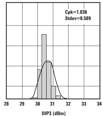
Figure 4. OIP3 @ 2.7 V, 10 mA. LSL = 22.0, Nominal = 24.2
