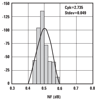
Figure 2. NF @ 2.7 V, 10 mA. USL = 0.9, Nominal = 0.6
