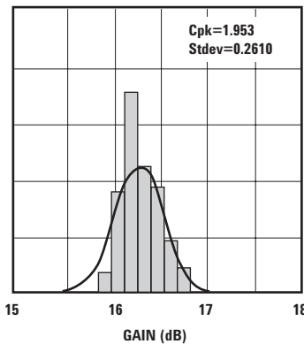
Figure 3. Gain @ 2.7 V, 10 mA. USL = 18.5, LSL = 15.5, Nominal = 17.7
