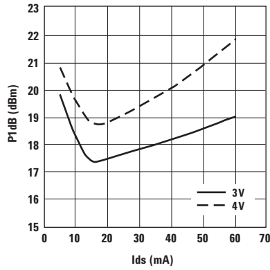
Figure 14. P1dB vs. Idsq and Vds Tuned for Max OIP3 and Fmin at 900 MHz. [1]
