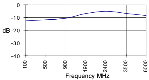
S22, Id =12mA, T=-40C
