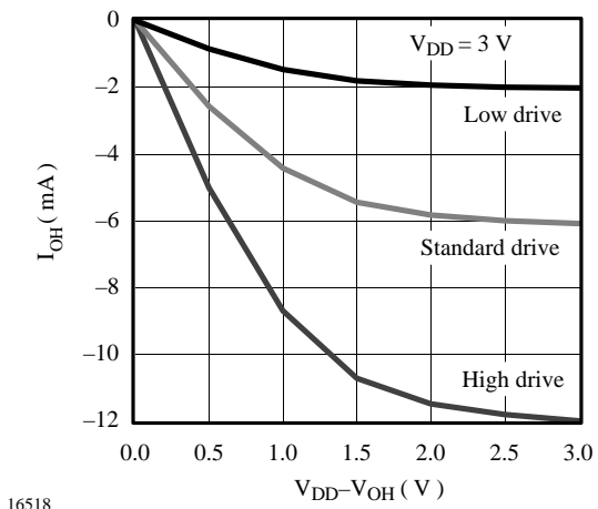
Figure 56. Typical high output driver
