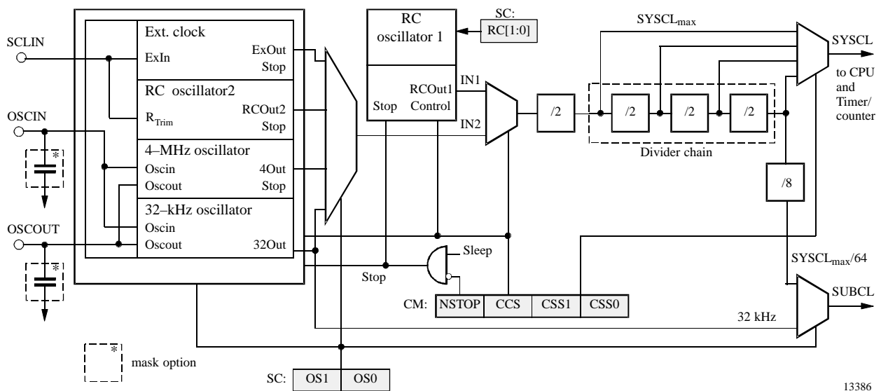
Figure 10. Clock module
