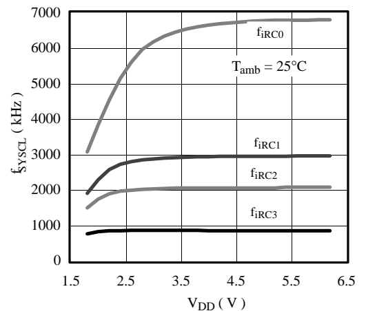
Figure 53. f_{SYSCL} = f(V_{DD}); internal RC
