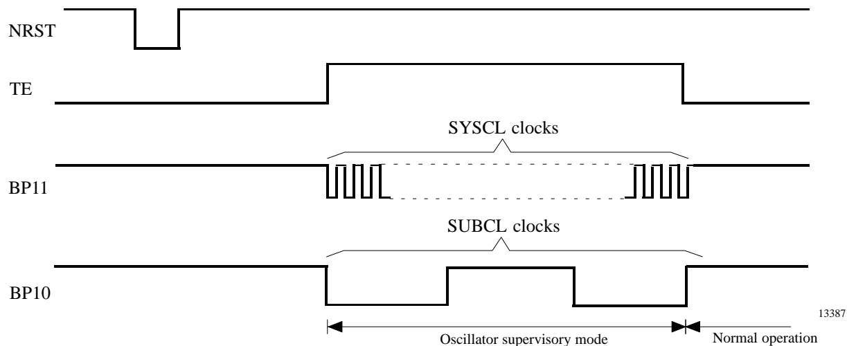
Figure 16. Clock monitoring
