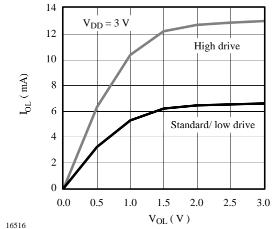
Figure 57. Typical low output driver
