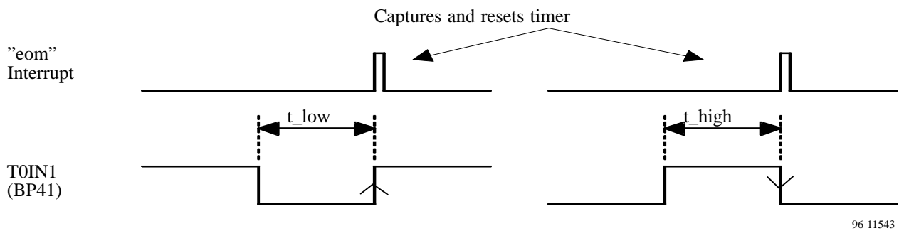
Figure 37. Pulse width measurement
