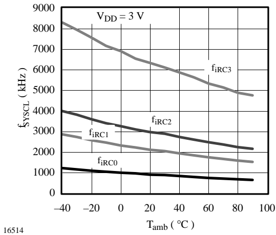
Figure 54. f_{SYSCL} = f(T_{amb})
