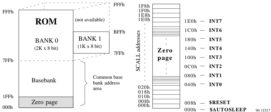
Figure 4. ROM map of M44C510E
