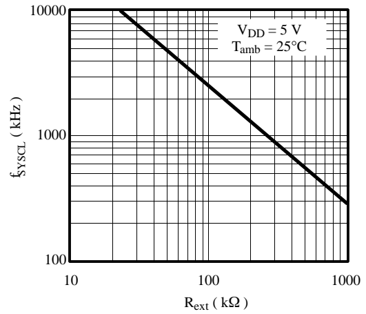
Figure 51. f_{SYSCL} = f(R_{ext})
