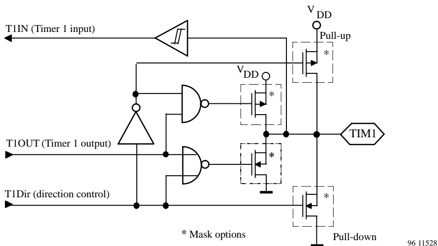
Figure 24. Bidirectional pin TIM1
