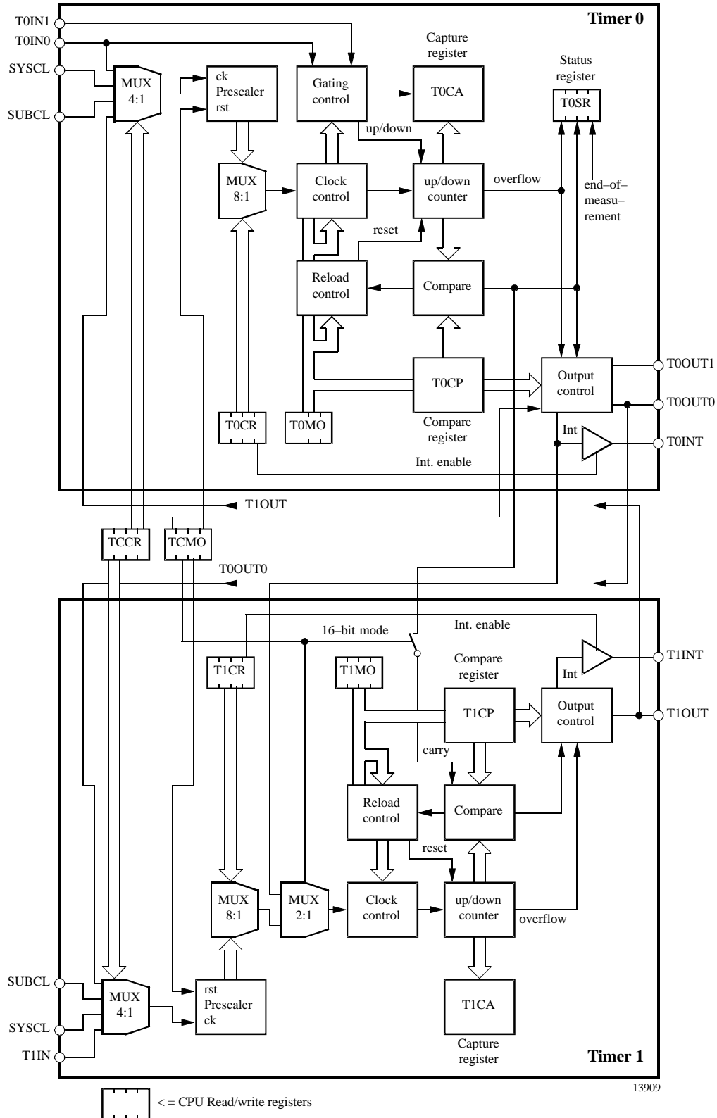
Figure 27. Timer/counter module
