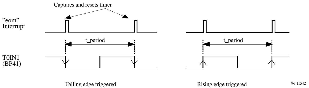
Figure 36. Period measurement
