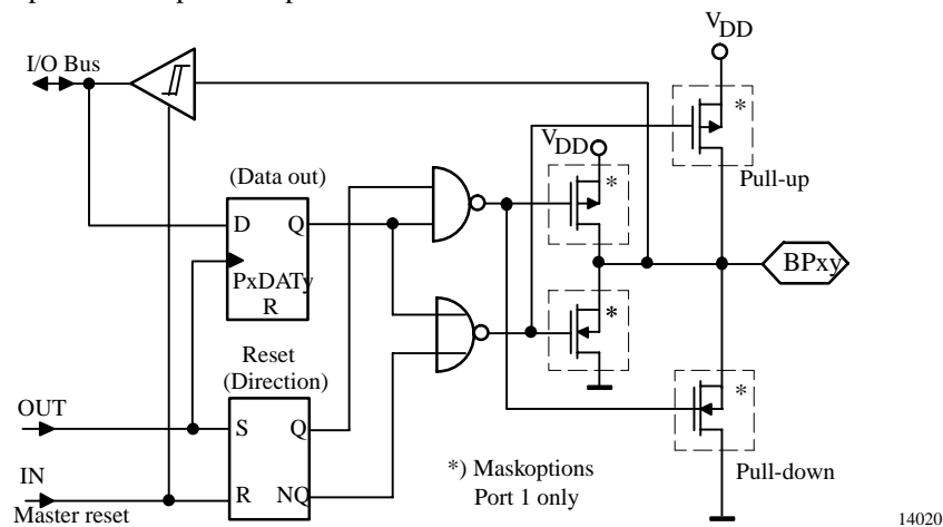
Figure 18. Bidirectional Ports 0 and 1
