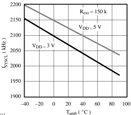
Figure 50. f_{SYSCL} = f(T_{amb}); external RC
