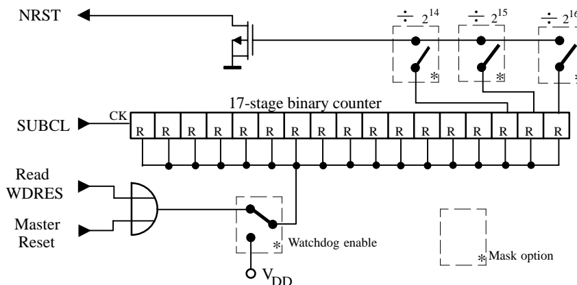
Figure 26. Watchdog timer
