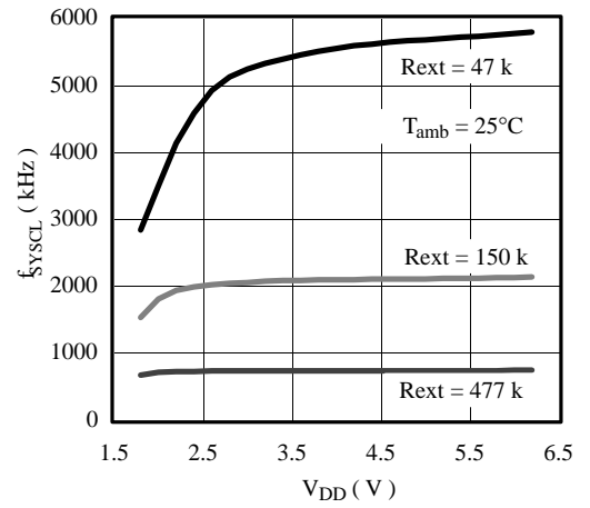
Figure 52. f_{SYSCL} = f(V_{DD}, R_{ext})
