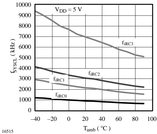
Figure 55. f_{SYSCL} = f(T_{amb})
