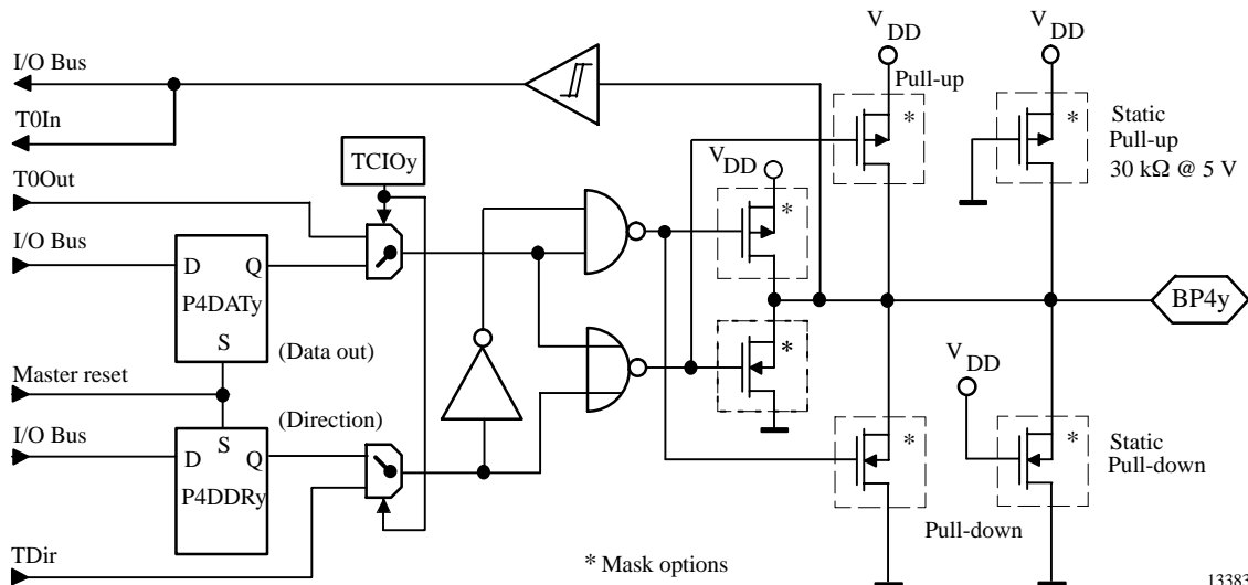
Figure 23. Bidirectional Port 4
