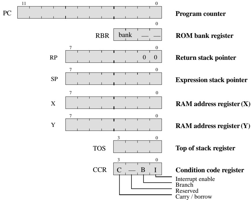
Figure 6. Programming model
