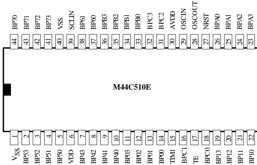
Figure 2. Pin connections SSO44-package
