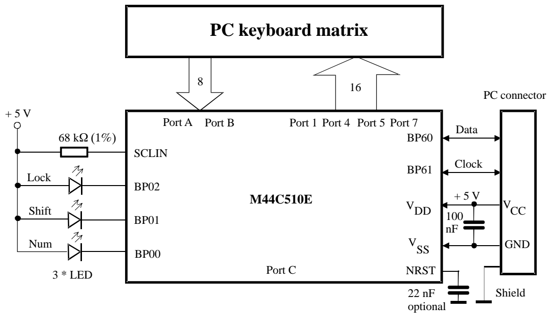
Figure 62. M44C510E as keyboard controller
