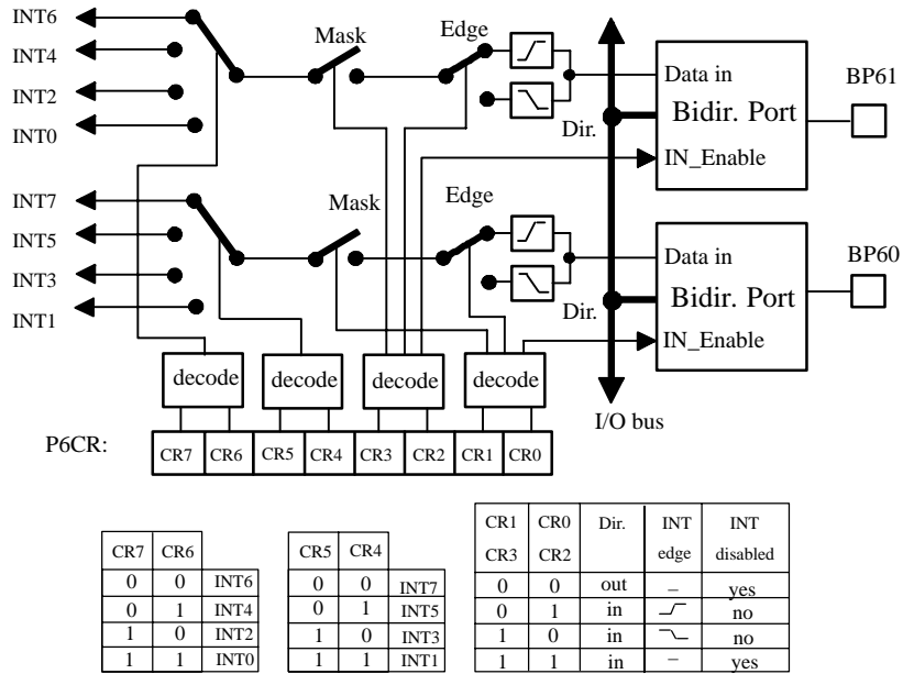
Figure 22. Port 6 external interrupts
