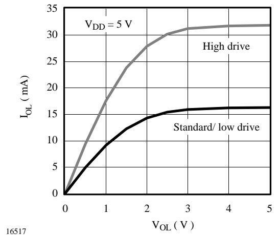
Figure 58. Typical low output driver
