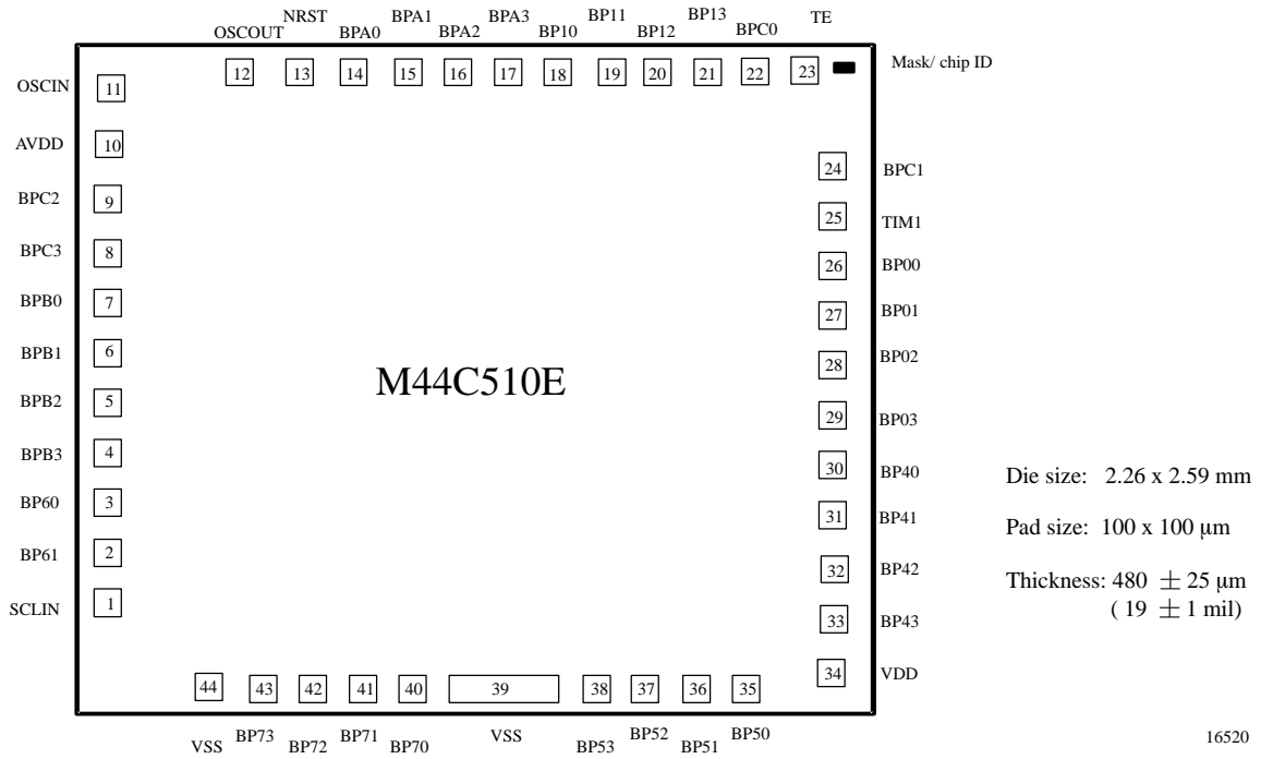
Figure 60. Pad assignments
