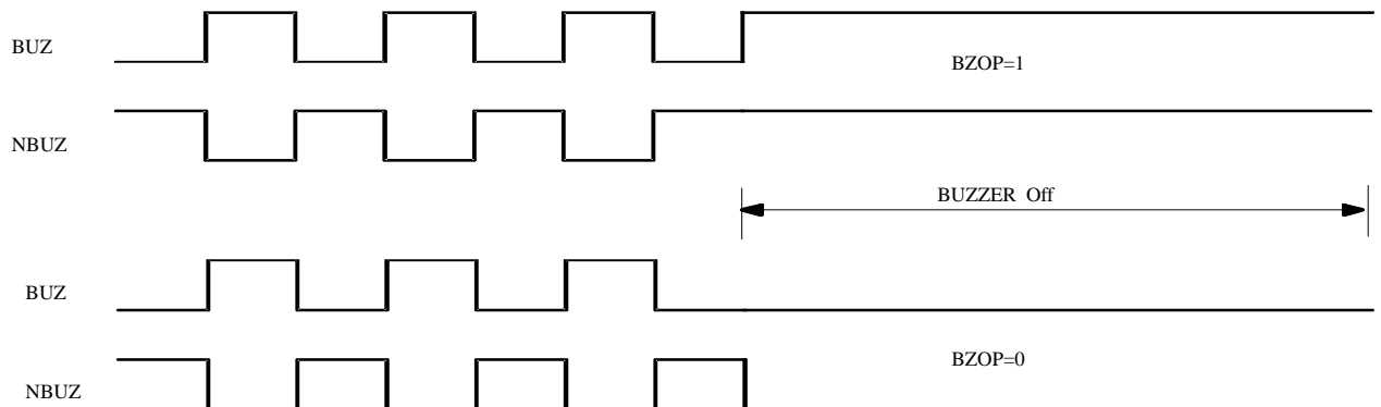
Figure 44. Buzzer waveform
