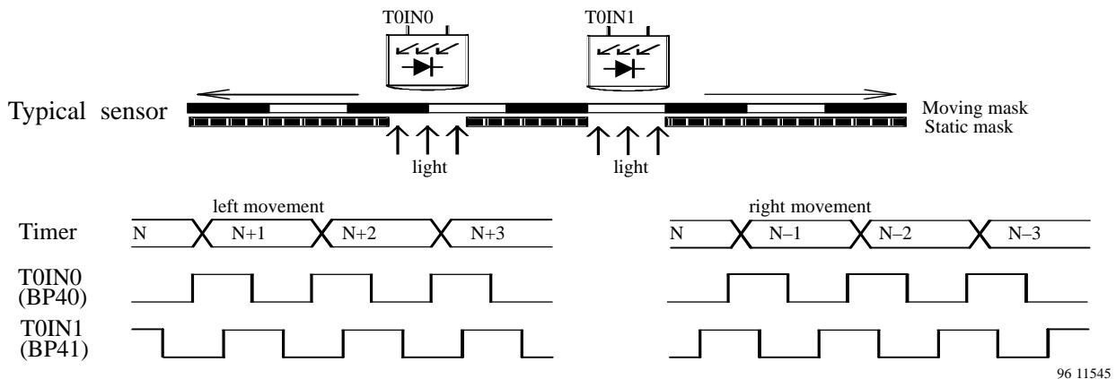
Figure 39. Position measurement mode
