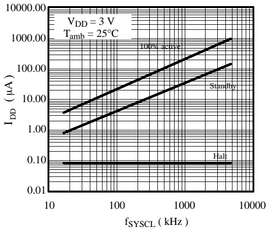
Figure 48. I_{DD} = f(f_{SYSCL})
