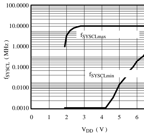
Figure 47. Worst case minimum/ maximum system frequency (using external RC or crystal oscillator)
