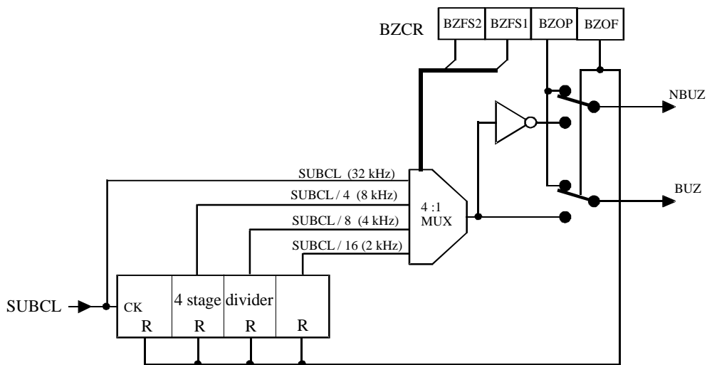
Figure 43. Buzzer module
