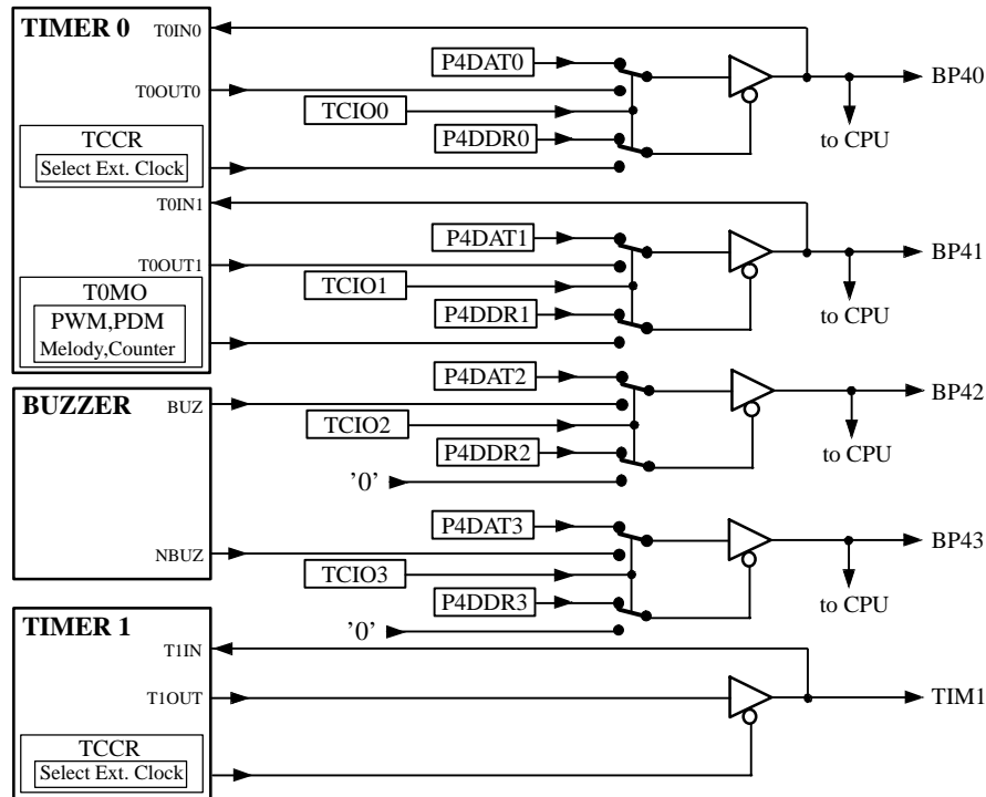
Figure 28. Timer/counter and buzzer external interface
