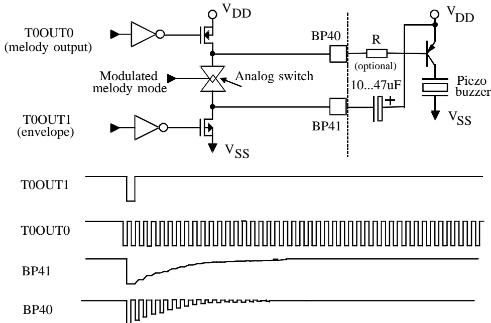
Figure 33. Modulated melody output circuit
