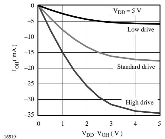
Figure 59. Typical high output driver
