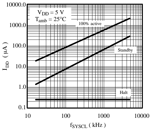
Figure 49. I_{DD} = f(f_{SYSCL})
