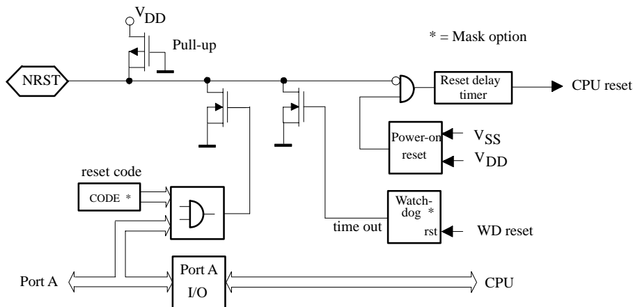
Figure 9. Reset configuration
