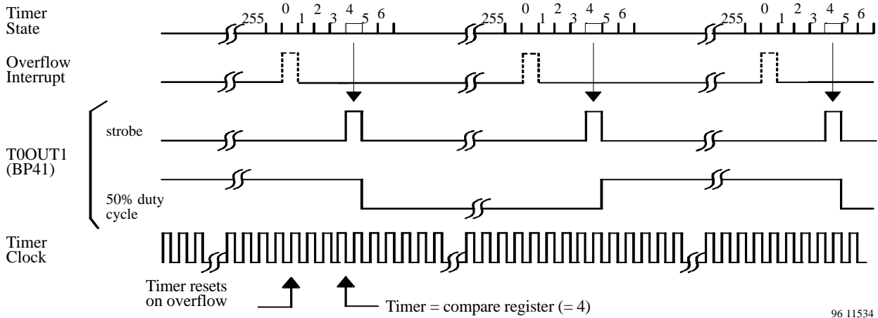
Figure 30. Timer 0 free running counter mode
