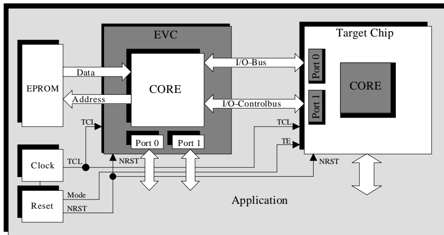
Figure 45. Emulation
