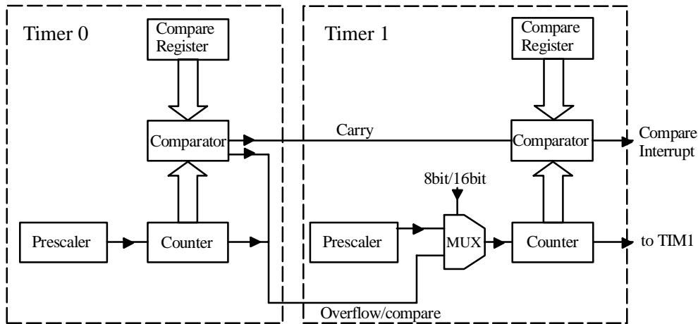
Figure 29. 16-bit mode
