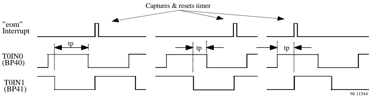
Figure 38. Phase measurement
