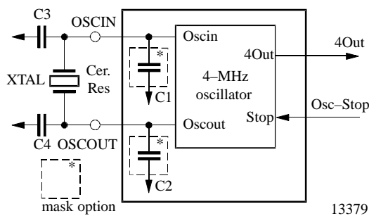
Figure 14. System clock oscillator
