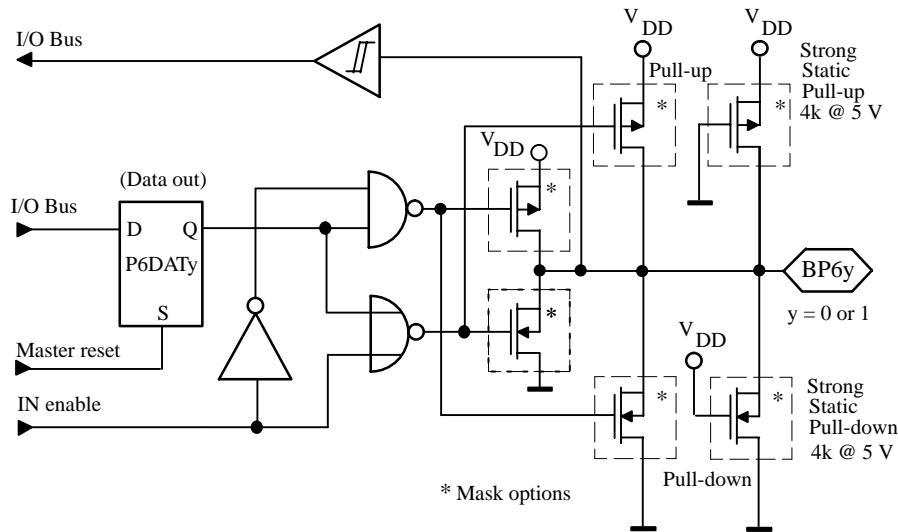
Figure 21. Bidirectional Port 6
