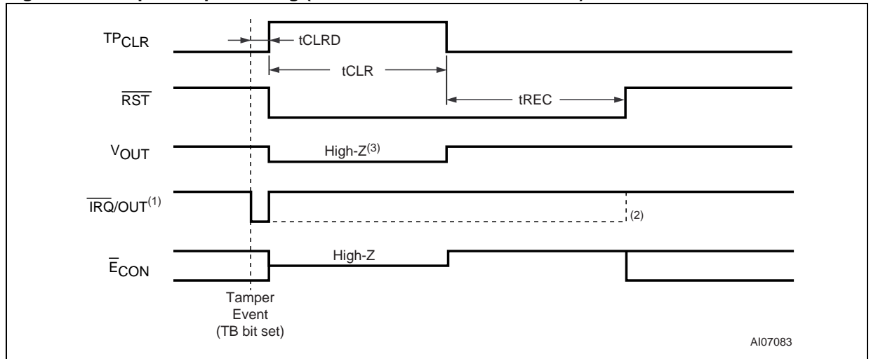
Figure 20. Tamper Output Timing (with CLR1EXT or CLR2EXT = '1')
