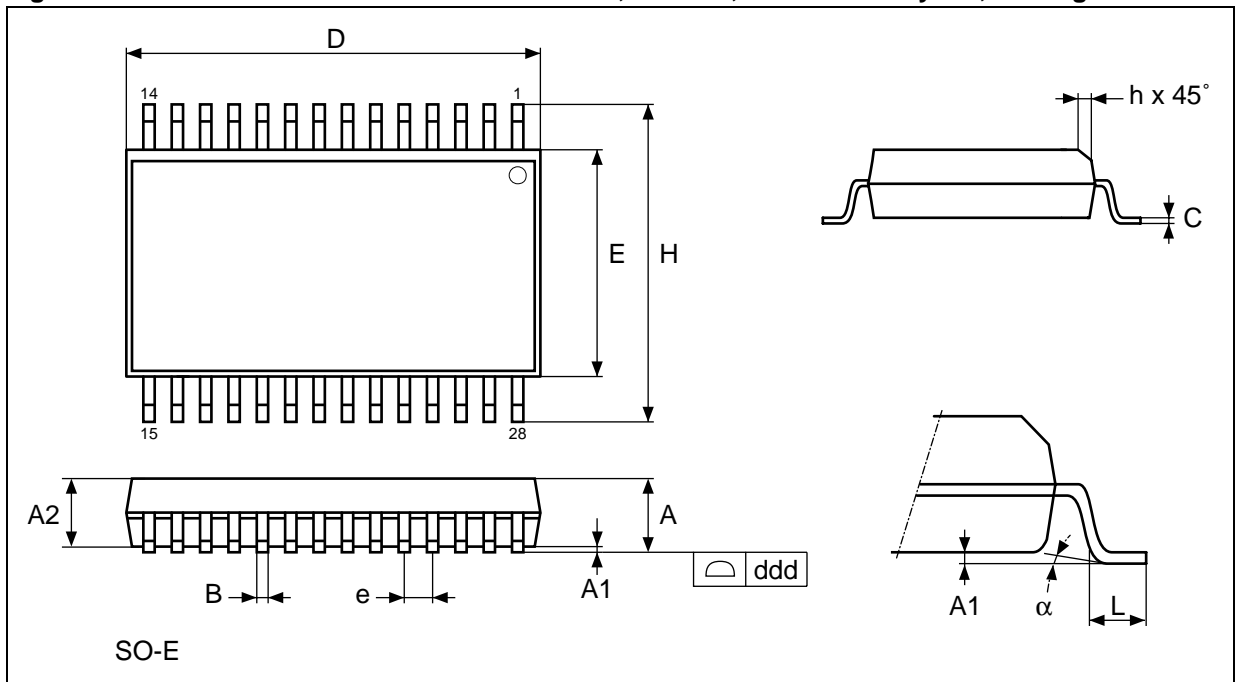
Figure 28. SOX28 – 28-lead Plastic Small Outline, 300mils, Embedded Crystal, Package Outline
