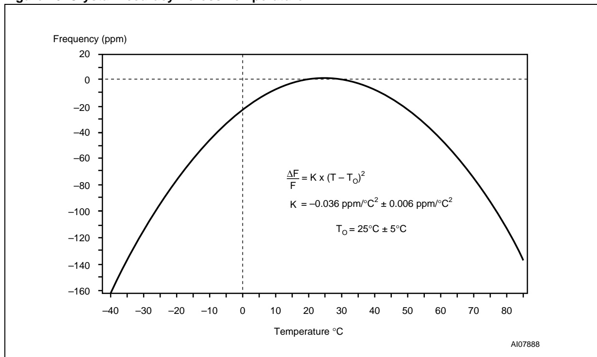
Figure 26. Crystal Accuracy Across Temperature
