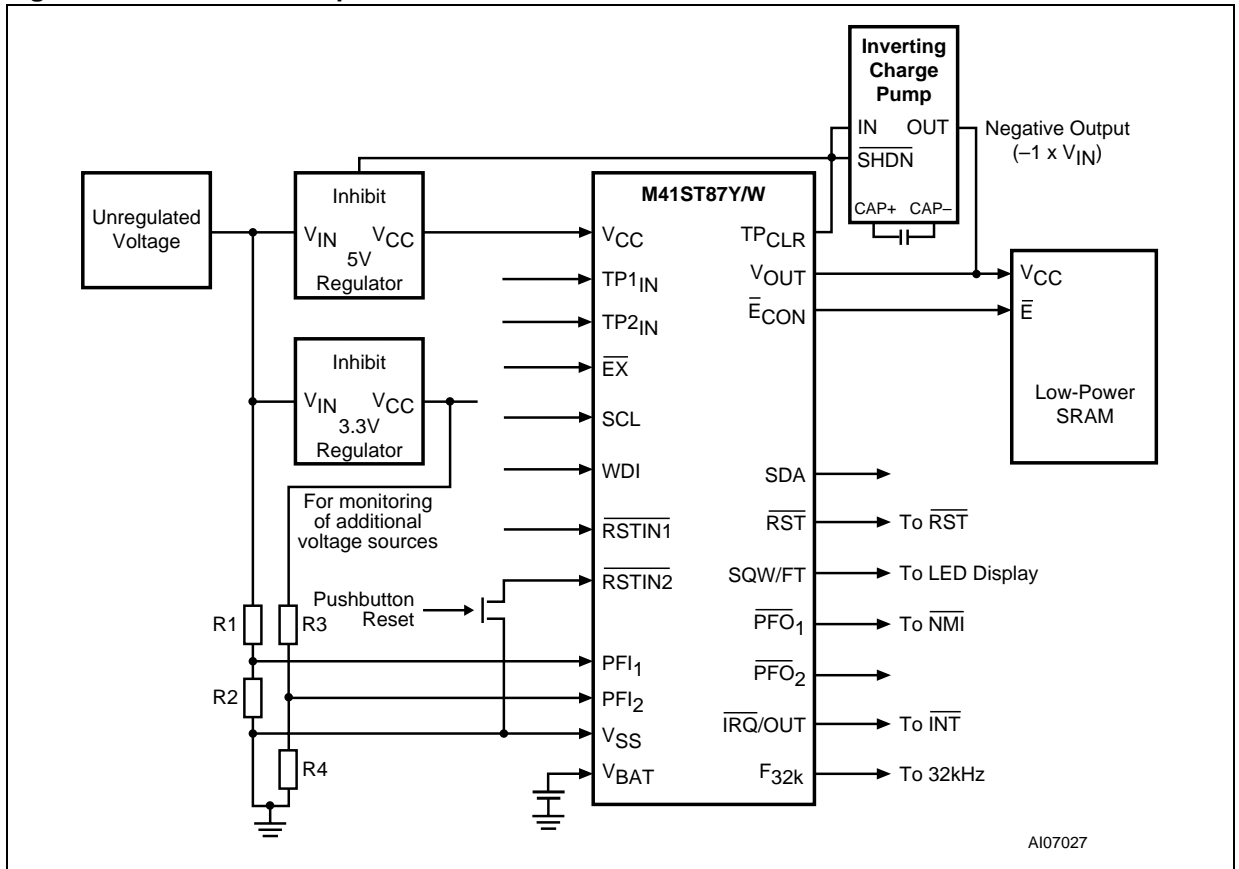
Figure 5. Hardware Hookup
