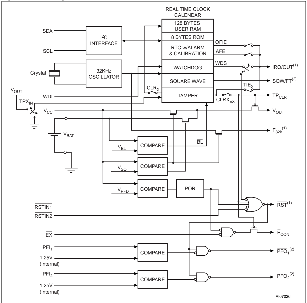
Figure 4. Block Diagram
