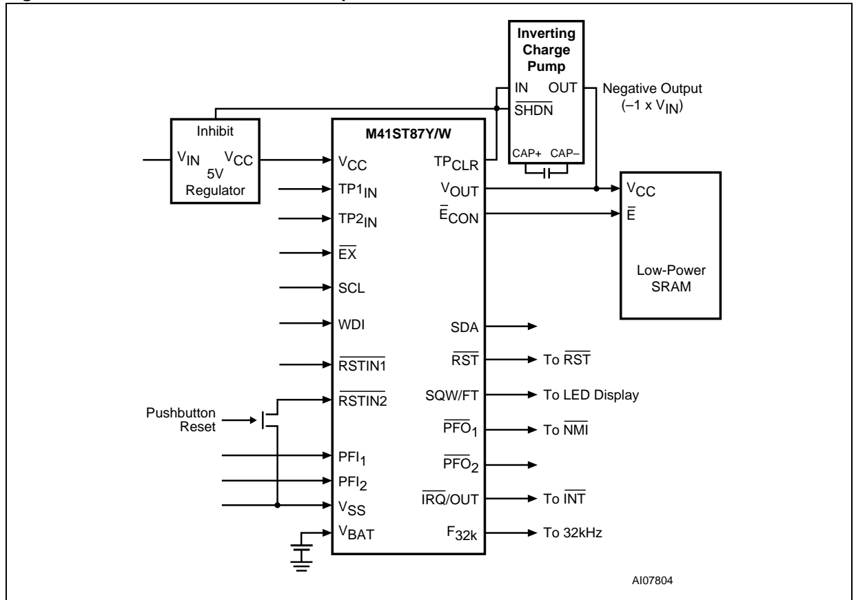
Figure 21. RAM Clear Hardware Hookup
