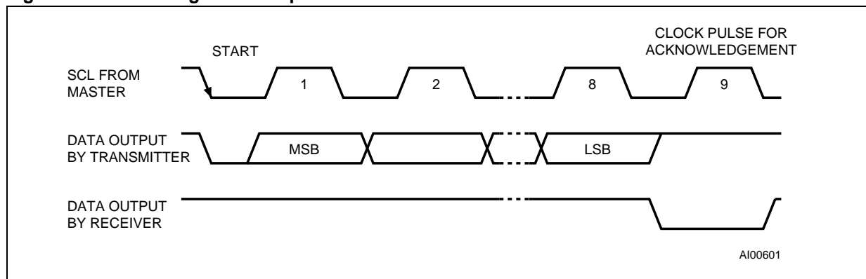
Figure 8. Acknowledgement Sequence
