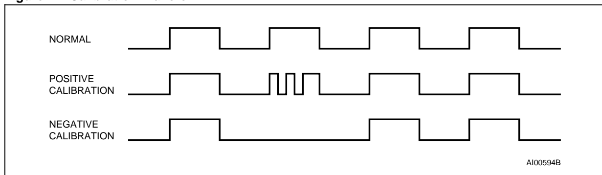
Figure 27. Calibration Waveform
