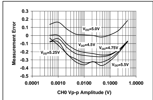
FIGURE 2-15: Measurement Error vs. V_{DD} ( G = 16 ).
