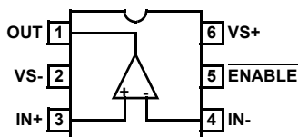
EL5100 (6 LD SOT-23) TOP VIEW
