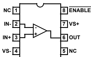
EL5100 (8 LD SO) TOP VIEW
