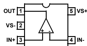
EL5101 (5 LD SOT-23) TOP VIEW
