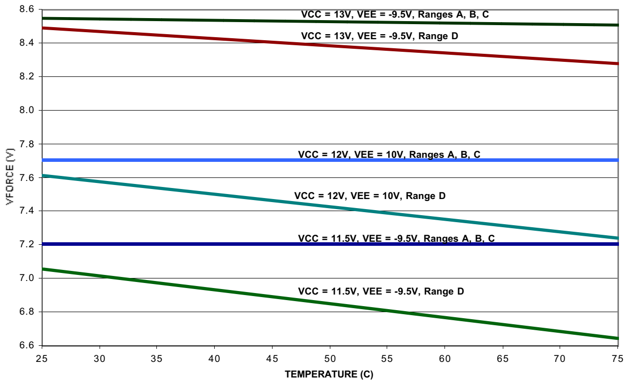
Edge 737 FORCE Voltage Positive Headroom
