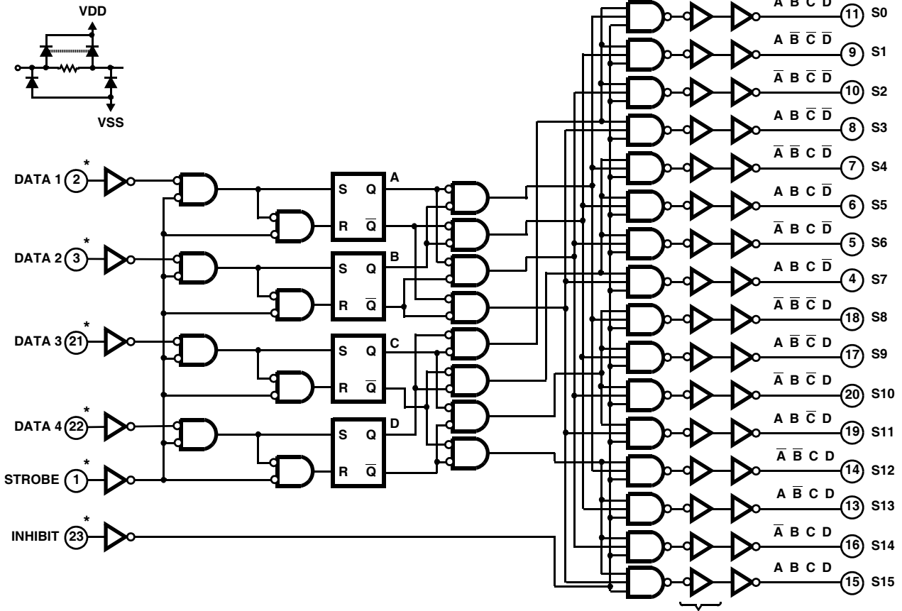
FIGURE 1. LOGIC DIAGRAM
