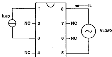
Fig. 3 - Leakage Current
