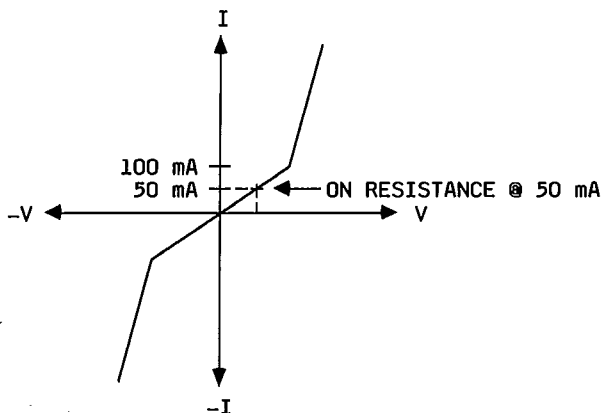
Fig. 5 - ON-State Characteristics of Output Poles (Illustrating Bidirectional V-I Characteristics)
