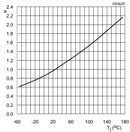
Fig 6. On-state resistance: typical values.
