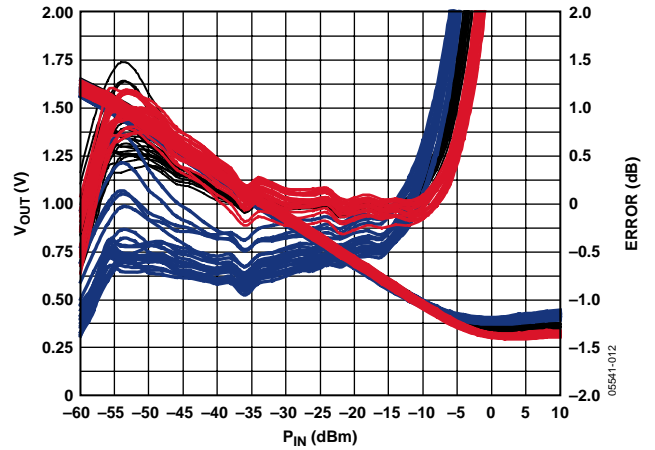
Figure 12. V_{OUT} and Log Conformance vs. Input Amplitude at 3.6 GHz, Multiple Devices, R_{TADJ} = 8\text{ k}\Omega
