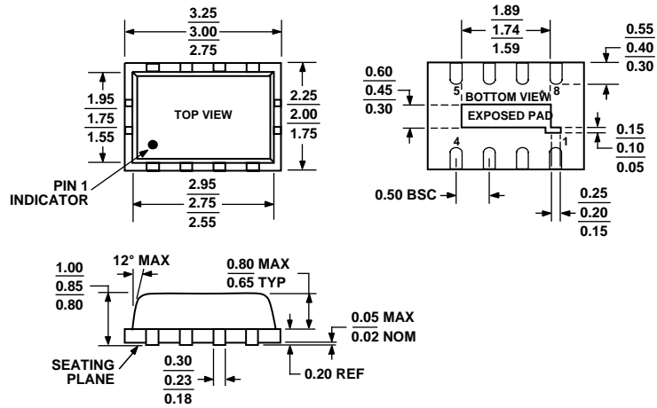
Figure 39. 8-Lead Lead Frame Chip Scale Package [LFCSP_VD] 2 mm x 3 mm Body, Very Thin, Dual Lead (CP-8-1) Dimensions shown in millimeters
