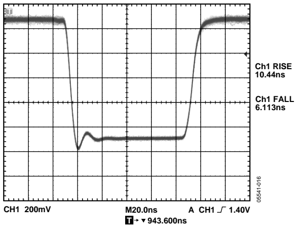
Figure 16. Power On/Off Response Time; V_P = 3.0 \text{ V} ; Input AC-Coupling Caps = 10 pF; C_{LPF} = \text{Open}
