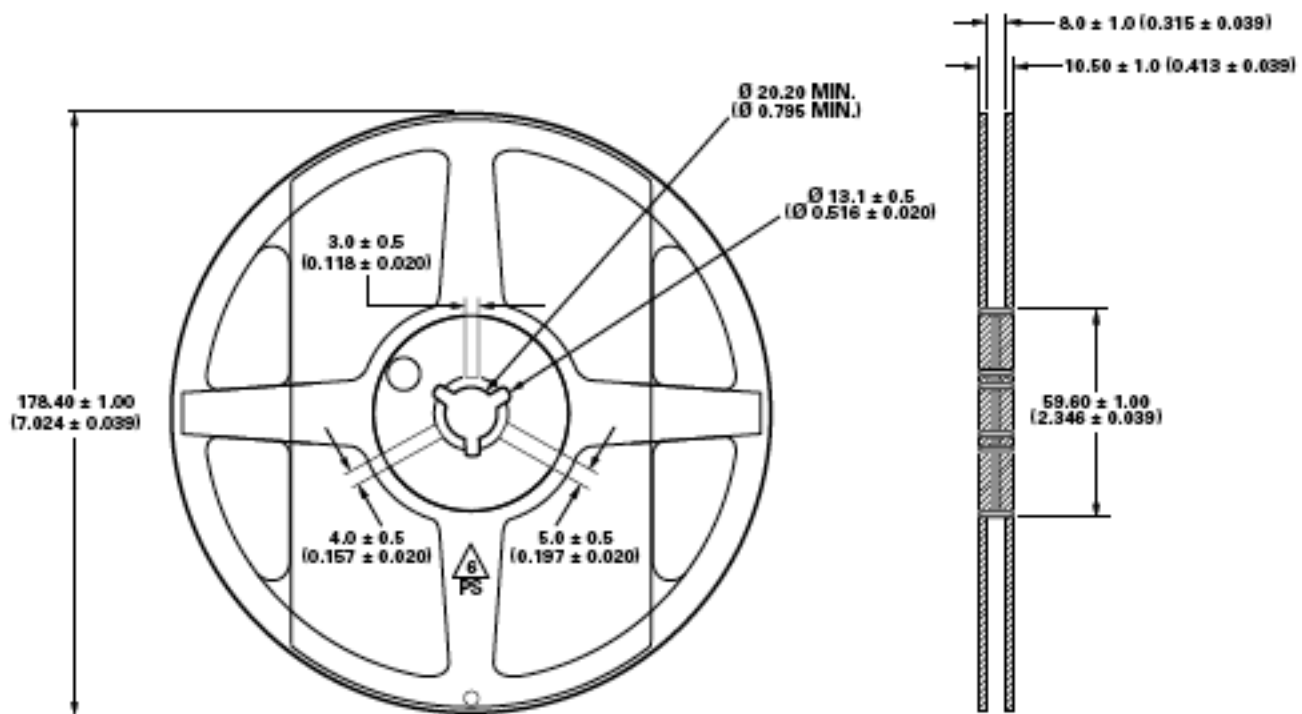
Figure 13. Reel dimensions.
