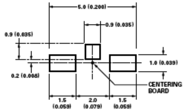
Figure 8. Recommended soldering pattern for HSMx-C110.
