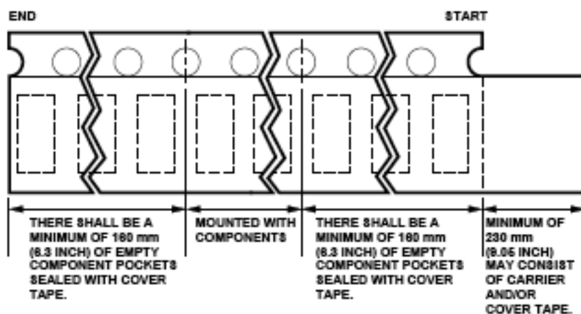
Figure 15. Tape leader and trailer dimensions.
