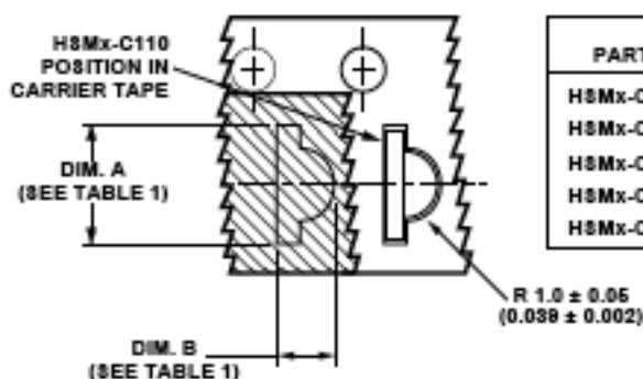
Figure 14. Tape dimensions.
