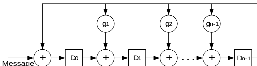
Figure 10: CRC Decoder
