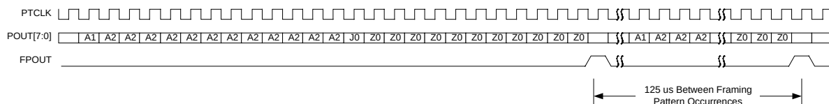
Figure 40: Parallel Transmit Interface Timing
