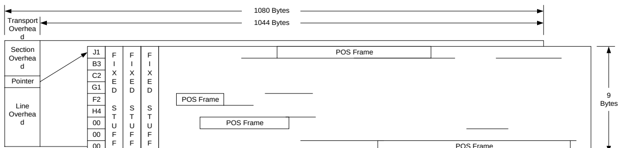
Figure 19: POS Mapping into the STS-12c/STM-4-4c SPE
