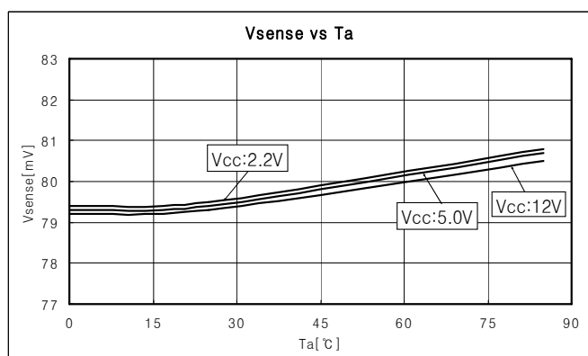
Fig.3 Vsense vs Ambient Temperature
