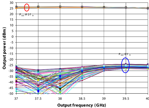
20DBL0629 (R10 C11): V dx2 =2.5V, V db =3 V, V dPA =4.5 V @ P in =0..+10 dBm
