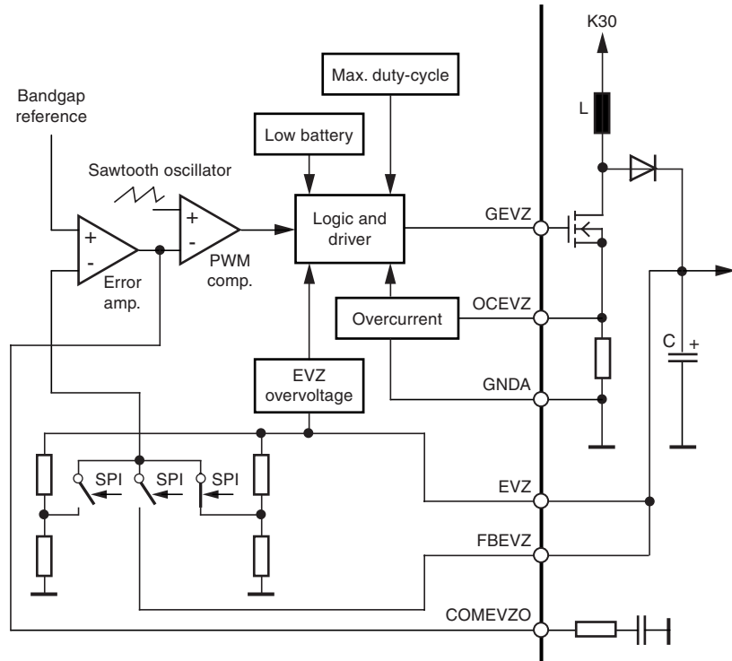
Figure 9-2. EVZ Regulator With Internal Divider
