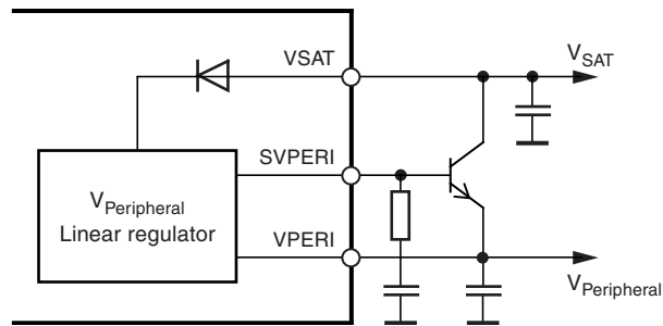
Figure 11-2. Functional Principle of the V_{\text{PERI}} Regulator With External Boost Transistor
