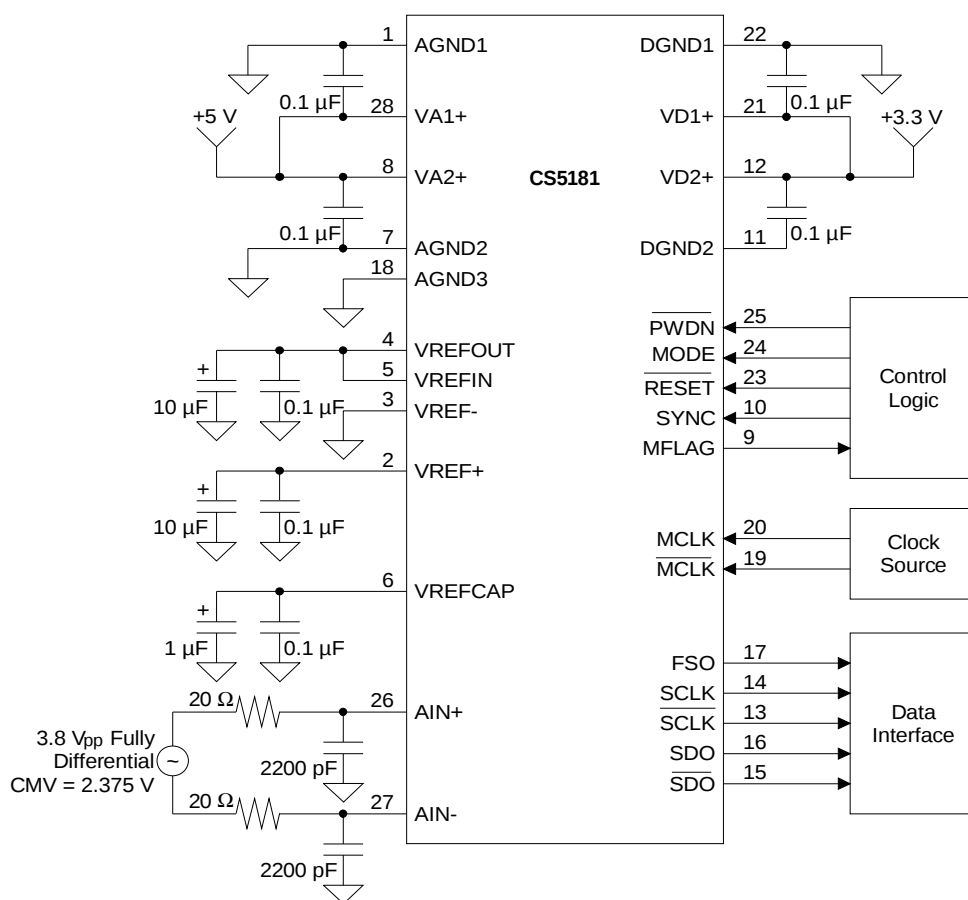
Figure 11. CS5181 System Connection Diagram
