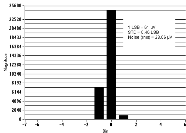
Figure 20. CS5181 Noise Histogram, 32768 samples.
