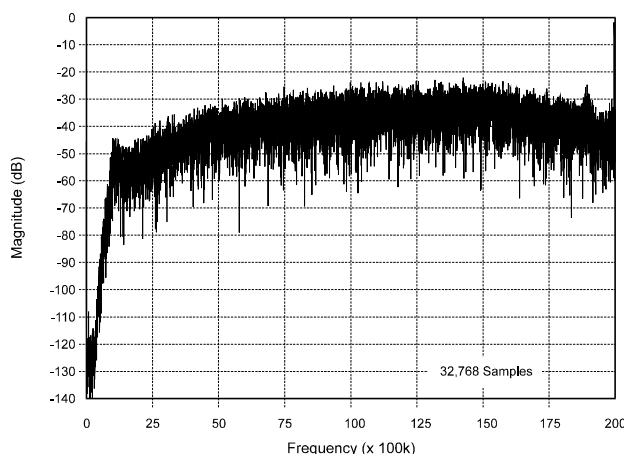
Figure 7. Magnitude versus frequency spectrum of modulator bitstream (MCLK = 40.0 MHz).
