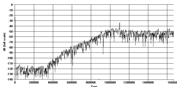
Figure 8. Expanded view of the magnitude versus frequency spectrum of modulator bitstream (MCLK = 40 MHz).
