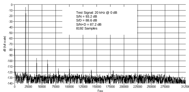
Figure 16. Performance of amplifier in Figure 15
