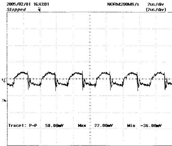
Figure 18 – 48 VDC, Full Load 3.3 V Output Ripple, 50 mV, 2 μs / div
