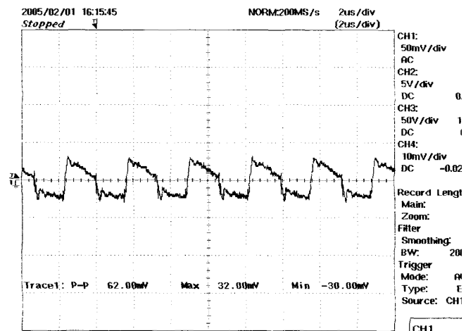
Figure 19 – 48 VDC, Full Load 5V Output Ripple, 50 mV, 2 μs / div
