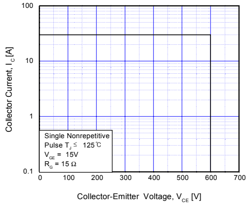
Fig 14. RBSOA Characteristics
