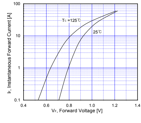
Fig 18. Rectifier ( Converter ) Characteristics
