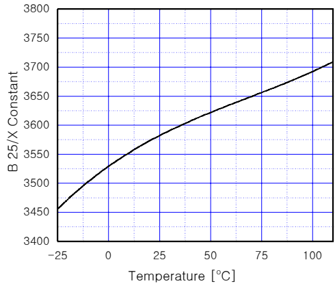
Fig 20. NTC Characteristics
