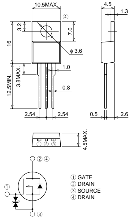
TO-220
