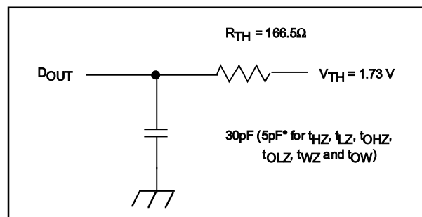
Figure 2. Thevenin Equivalent
