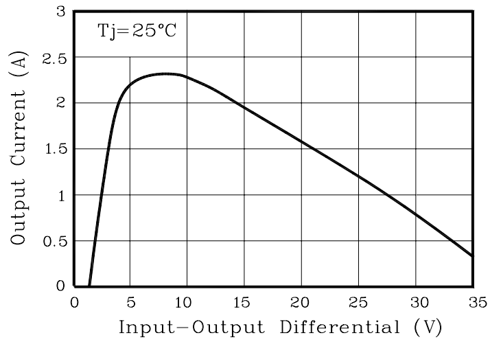
Fig. 2 I_{OUT} vs |V_{in} - V_{OUT}|
