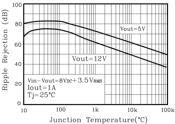
Fig. 5 Ripple Rejection
