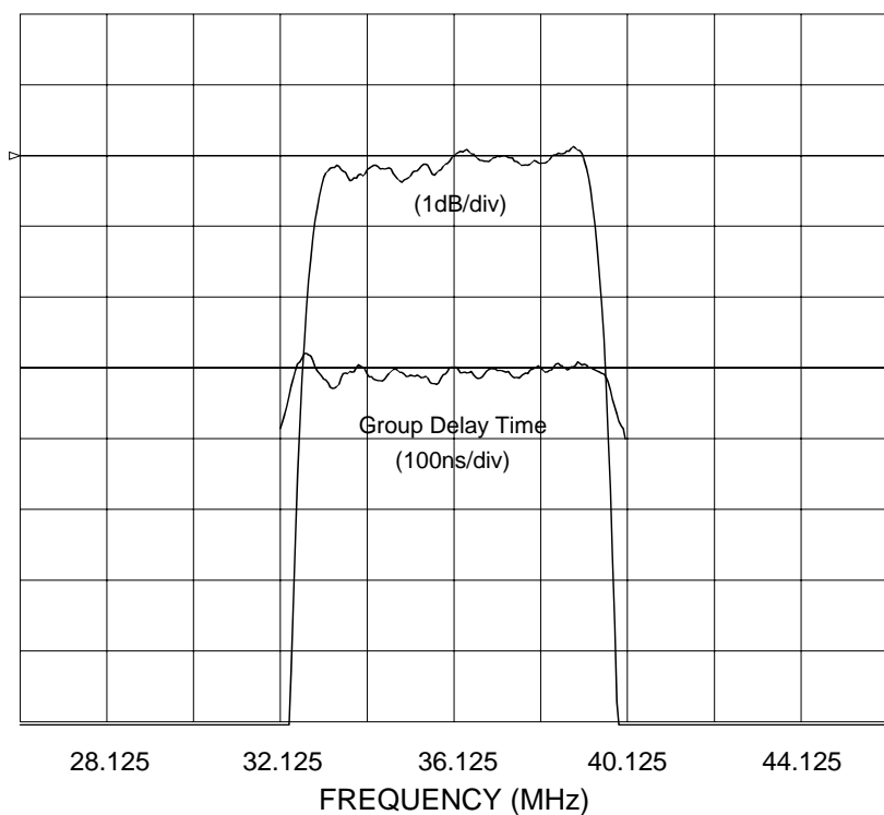
In-band Characteristics
