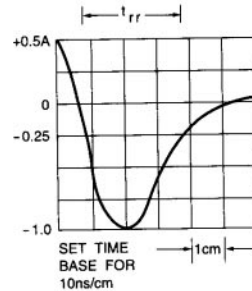
Fig. 5-REVERSE RECOVERY TIME CHARACTERISTIC AND TEST CIRCUIT DIAGRAM
