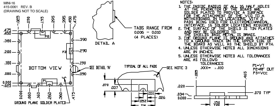
PHYSICAL DIMENSIONS
