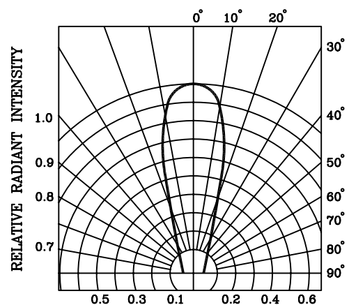
Fig.6 RADIATION DIAGRAM
