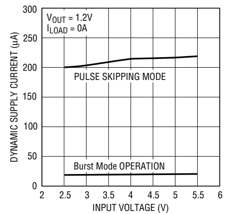
Dynamic Supply Current
