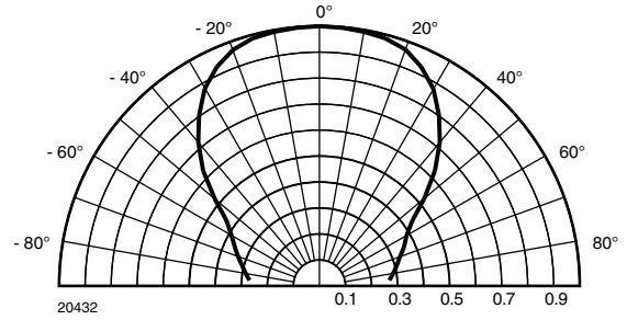
Fig. 12 - Directivity
