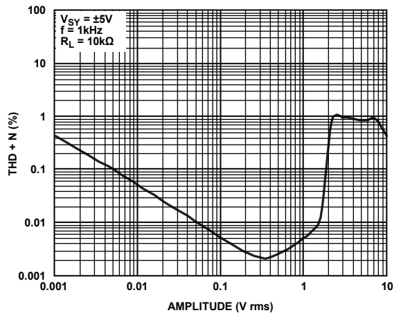
Figure 50. THD + N vs. Amplitude
