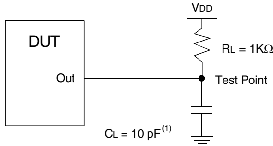
Load Circuit: PTYERR Output
