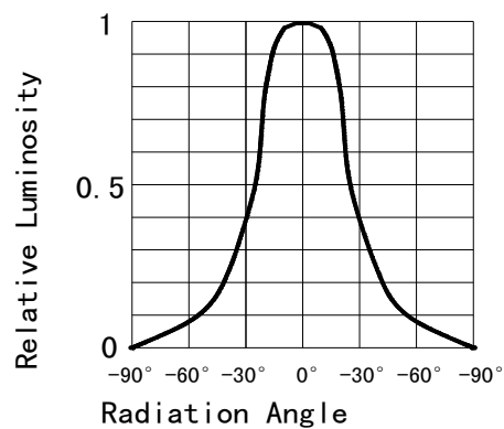
Fig 6. Relative Luminous Intensity vs. Radiation Angle
