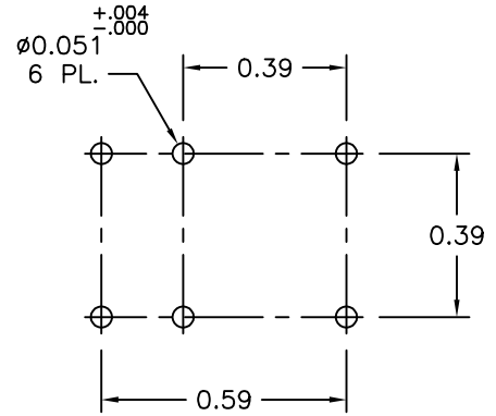
MOUNTING HOLES
