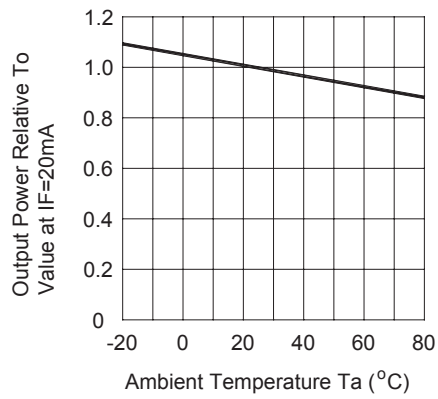
Figure 4. RELATIVE RADIANT INTENSITY VS. AMBIENT TEMPERATURE
