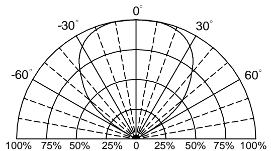
Fig.6 Directive Radiation
