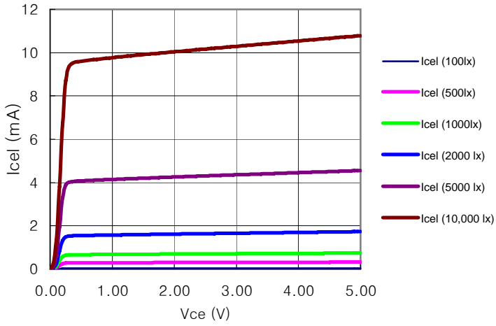
Collector current Vs. Collector - Emitter voltage T_a=25^\circ
