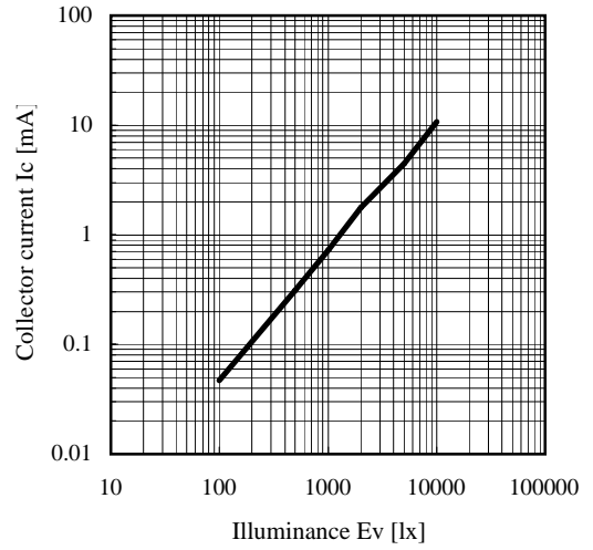
Collector current Vs. Illuminance V_{ce}=5V
