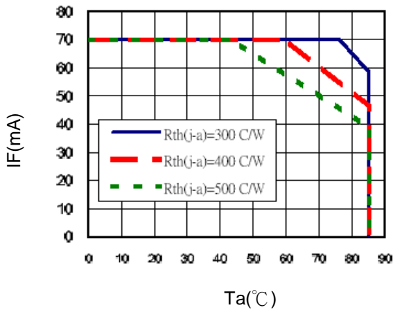
Fig.3 Derating curve based on T_j(\max)125^{\circ}\text{C}
