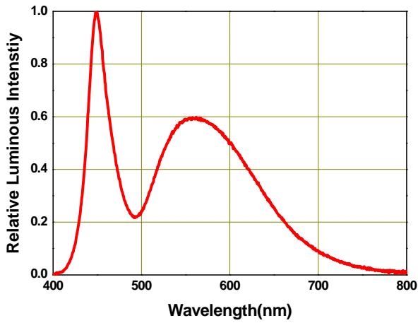
Relative Spectral Distribution, I_F=150\text{mA} , T_{\text{soldering}}=25^\circ\text{C}
