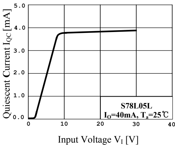
Fig.5 I_{QC} vs. V_I
